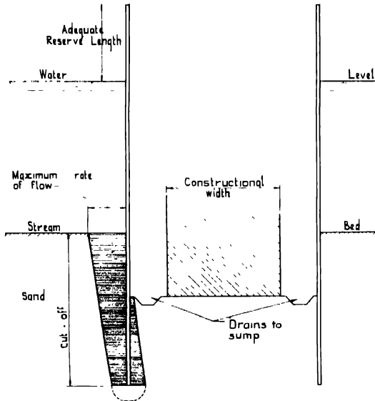
Fig. 152.—Sheet-Pile Cofferdam in Sand or similar Soil.
